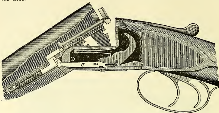
Baker's Split-slide Ejecting Mechanism.
